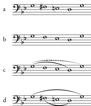
Figure 9: Some special cases in melodic minor.
