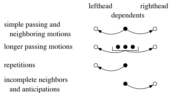
Figure 3: Four types of arc.
